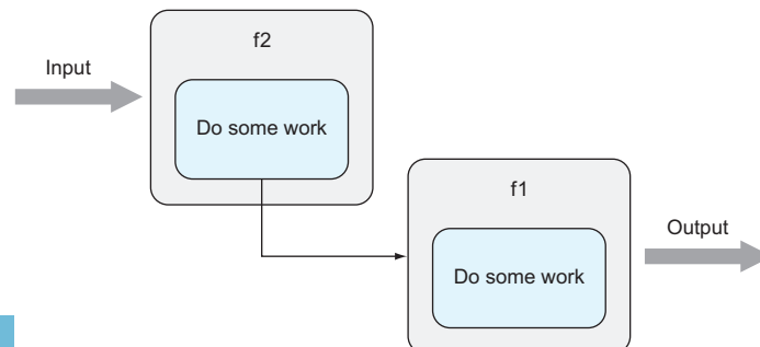
Figure 3.3 Chaining handlers
